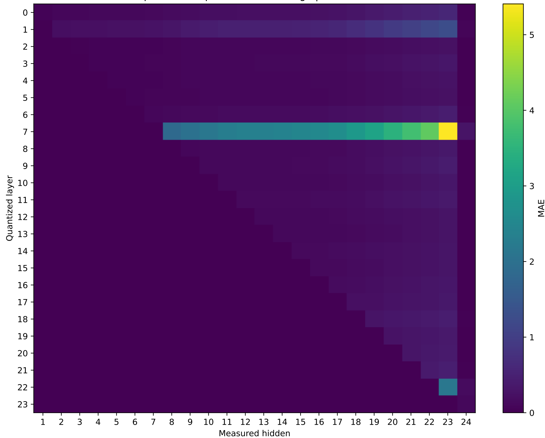
SmolLM2-1.7B-Instruct Prompt 4: MAE representation damage | float16 \rightarrow int8
