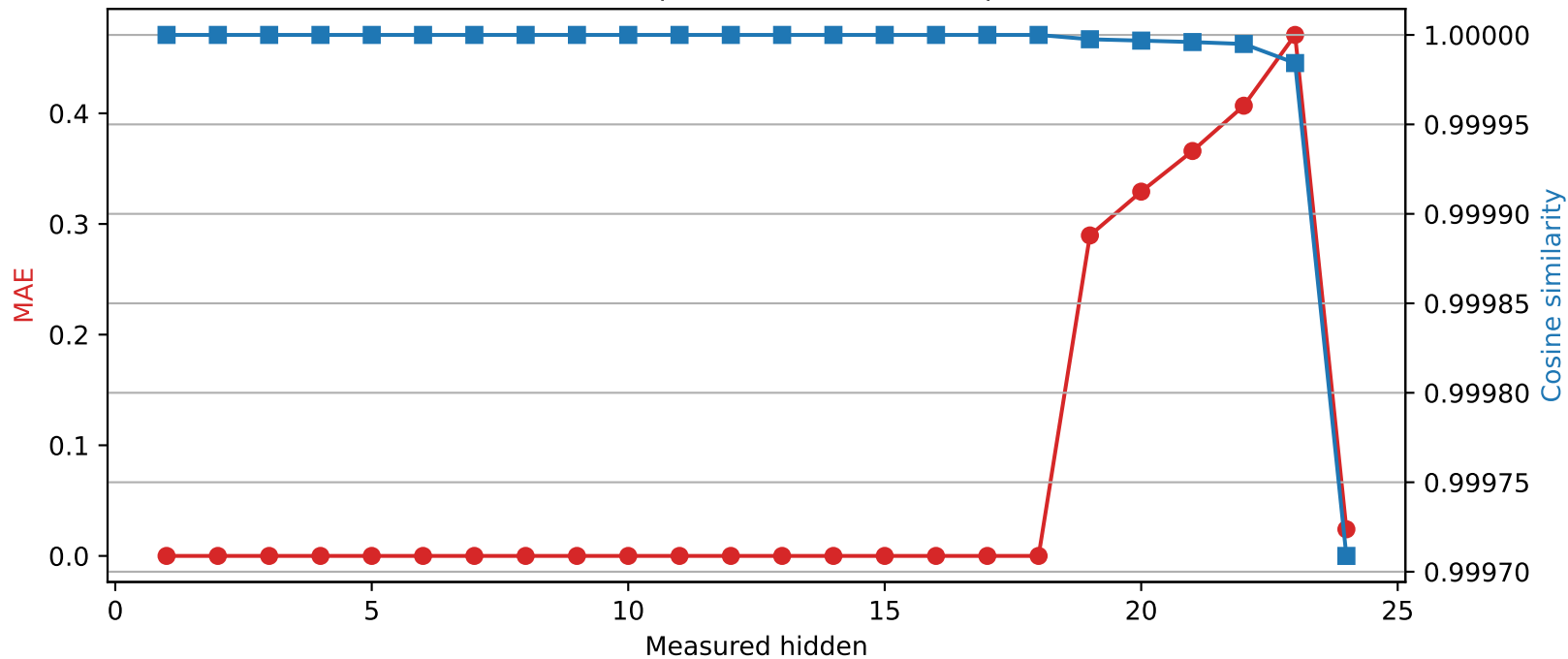
SmolLM2-1.7B-Instruct | Quantized layer 18 | float32 → int8
