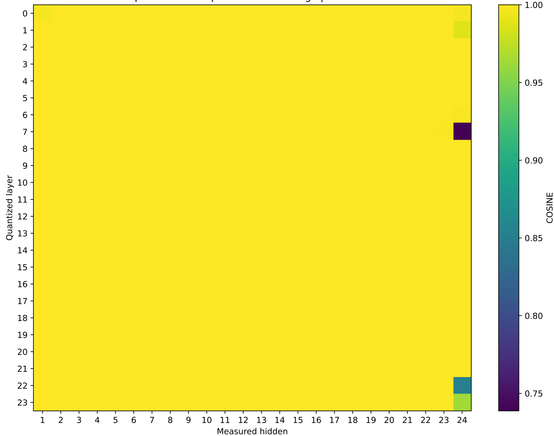
SmolLM2-1.7B-Instruct Prompt 0: cos sim representation damage | float64 → int8
