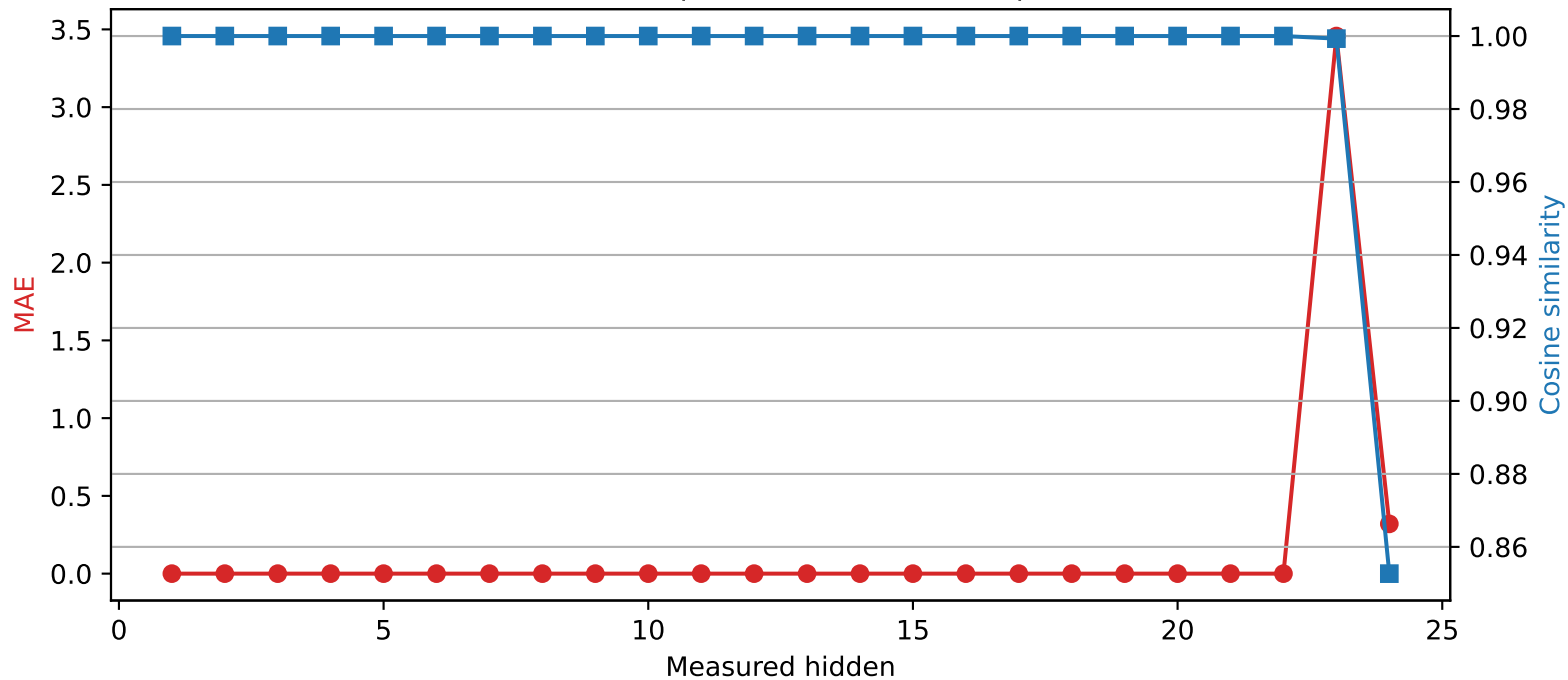
SmolLM2-1.7B-Instruct | Quantized layer 22 | float64 → int8
