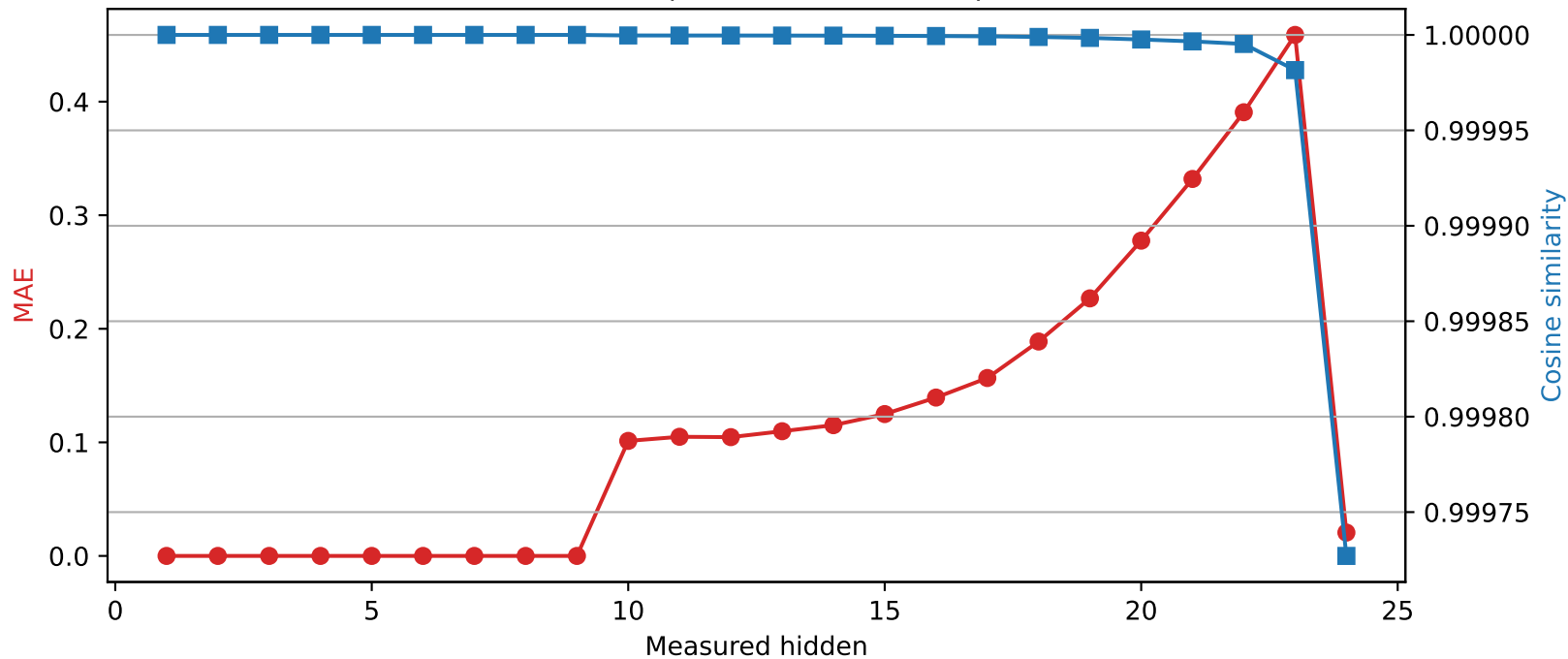
SmolLM2-1.7B-Instruct | Quantized layer 9 | float64 → int8
