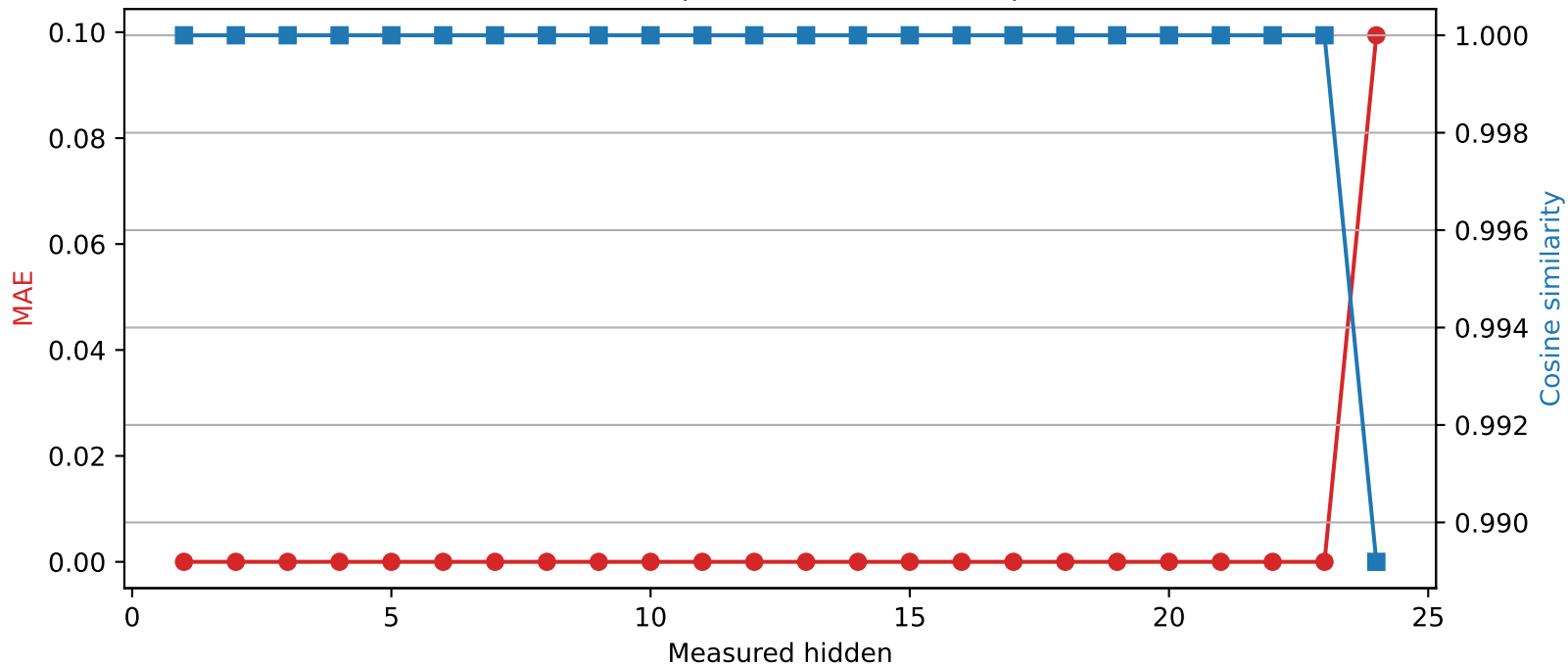
SmolLM2-1.7B-Instruct | Quantized layer 23 | float64 → int8
