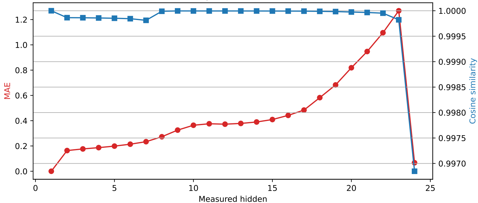
SmolLM2-1.7B-Instruct | Quantized layer 1 | float64 → int8
