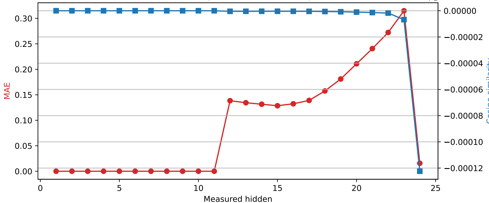
SmolLM2-1.7B-Instruct | Quantized layer 11 | float64 → int8
