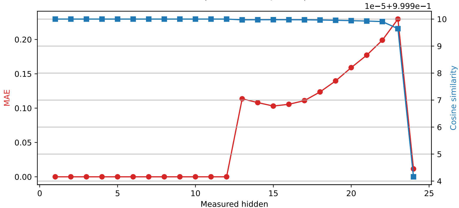
SmolLM2-1.7B-Instruct | Quantized layer 12 | float64 → int8
