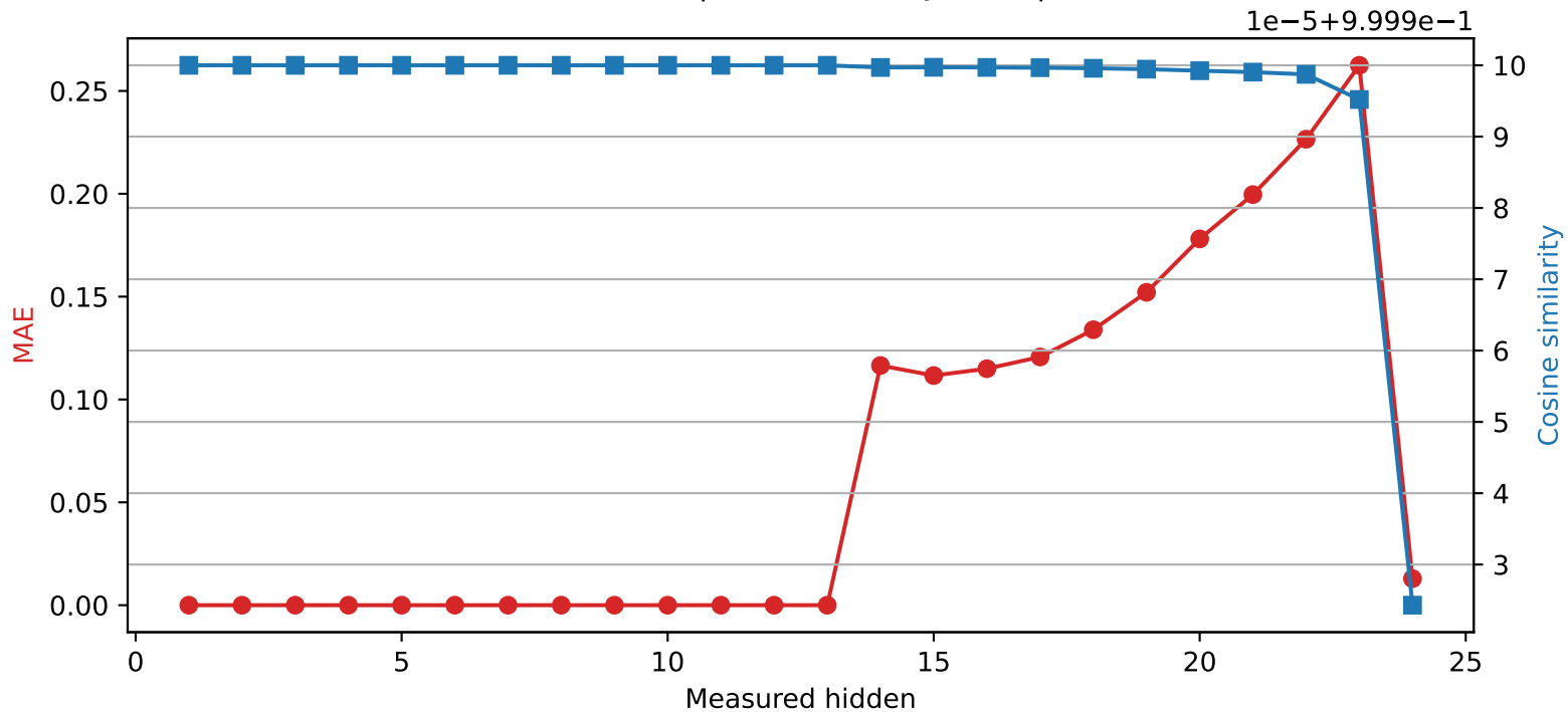
SmolLM2-1.7B-Instruct | Quantized layer 13 | float64 → int8
