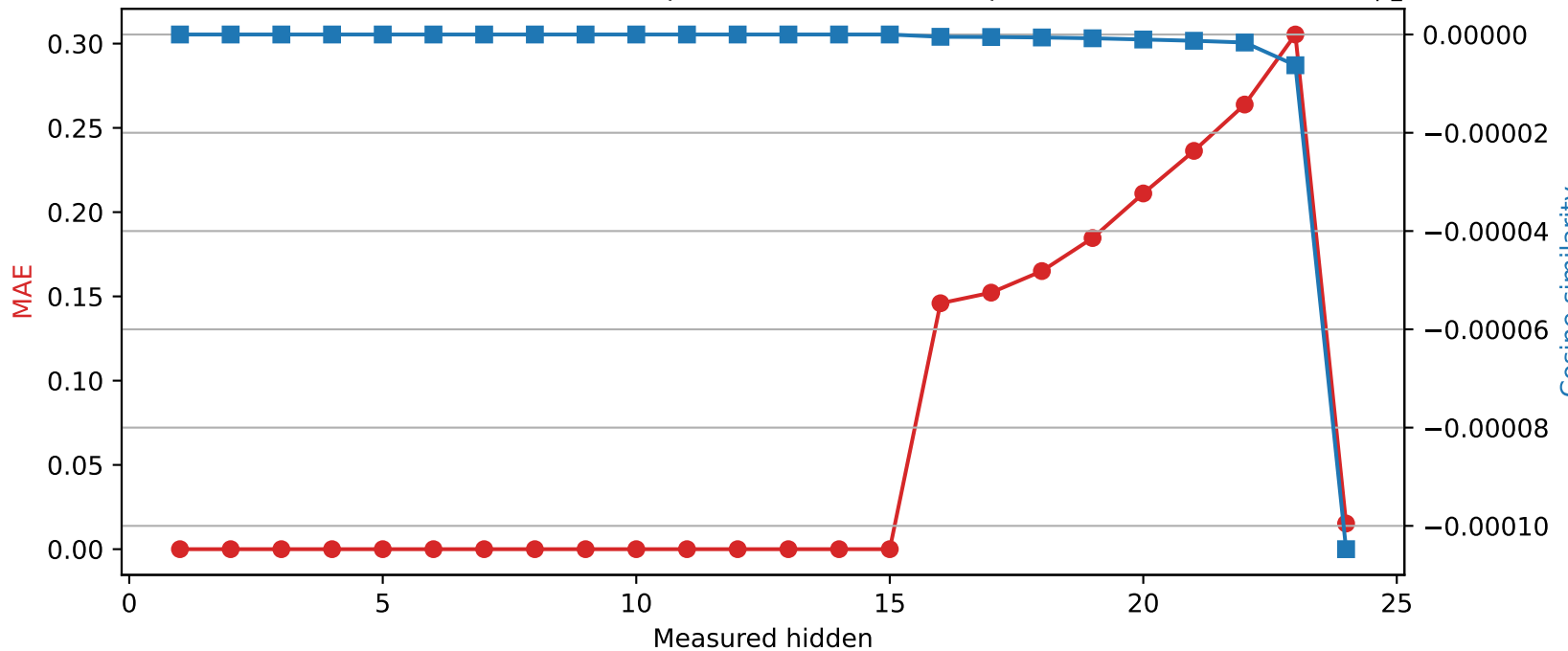
SmolLM2-1.7B-Instruct | Quantized layer 15 | float64 → int8
