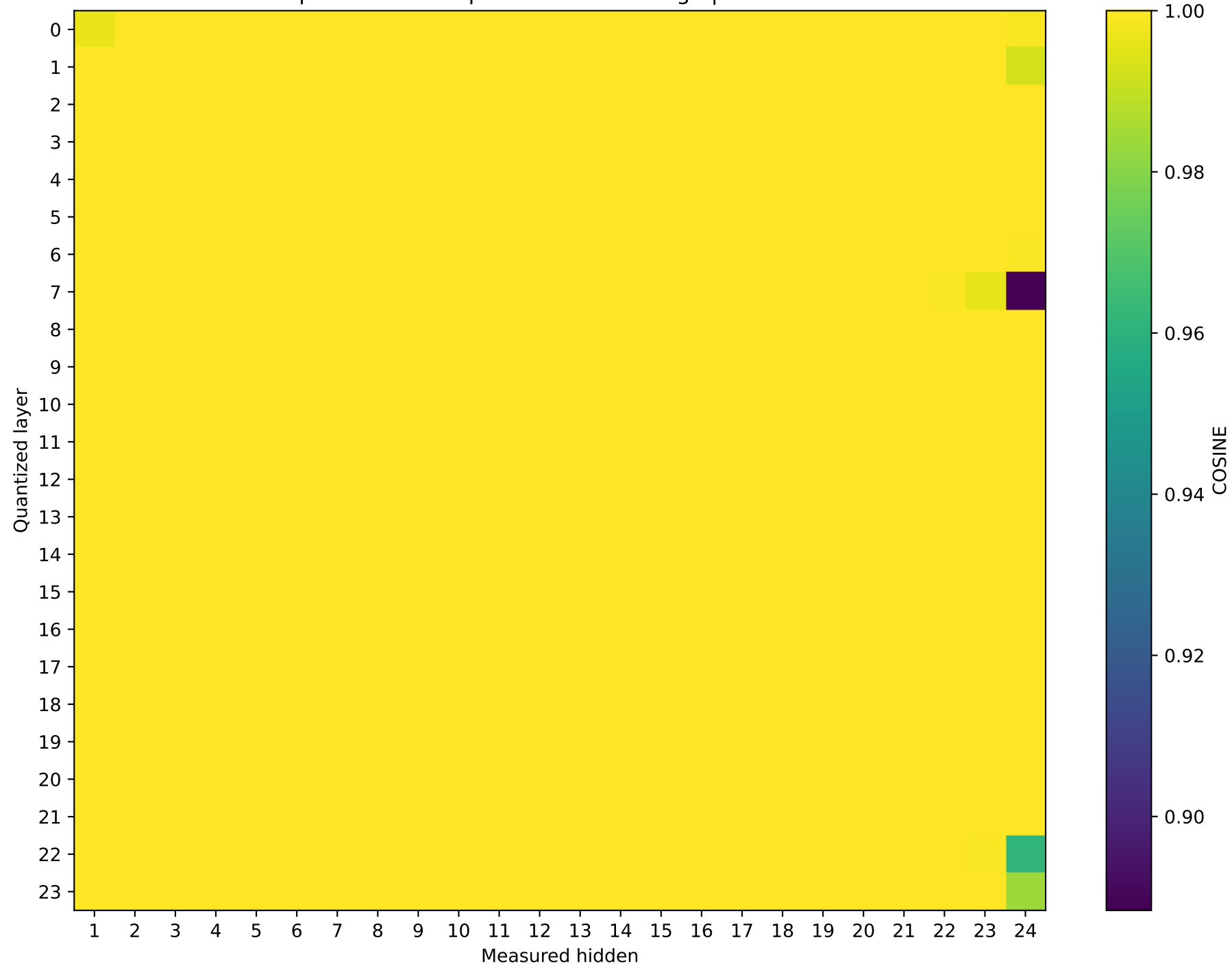
SmolLM2-1.7B-Instruct Prompt 3: cos sim representation damage | float64 → int8
