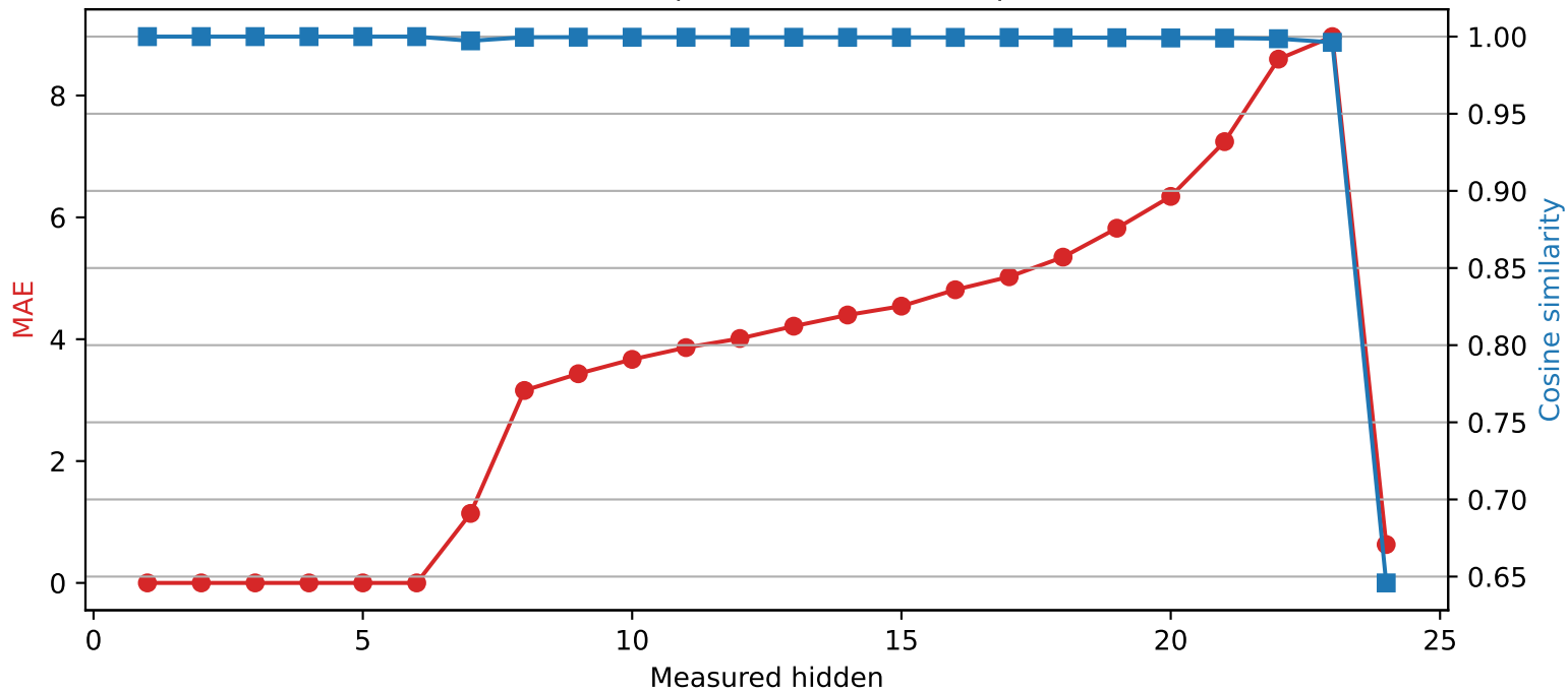
SmolLM2-1.7B-Instruct | Quantized layer 6 | float16 \rightarrow int4
