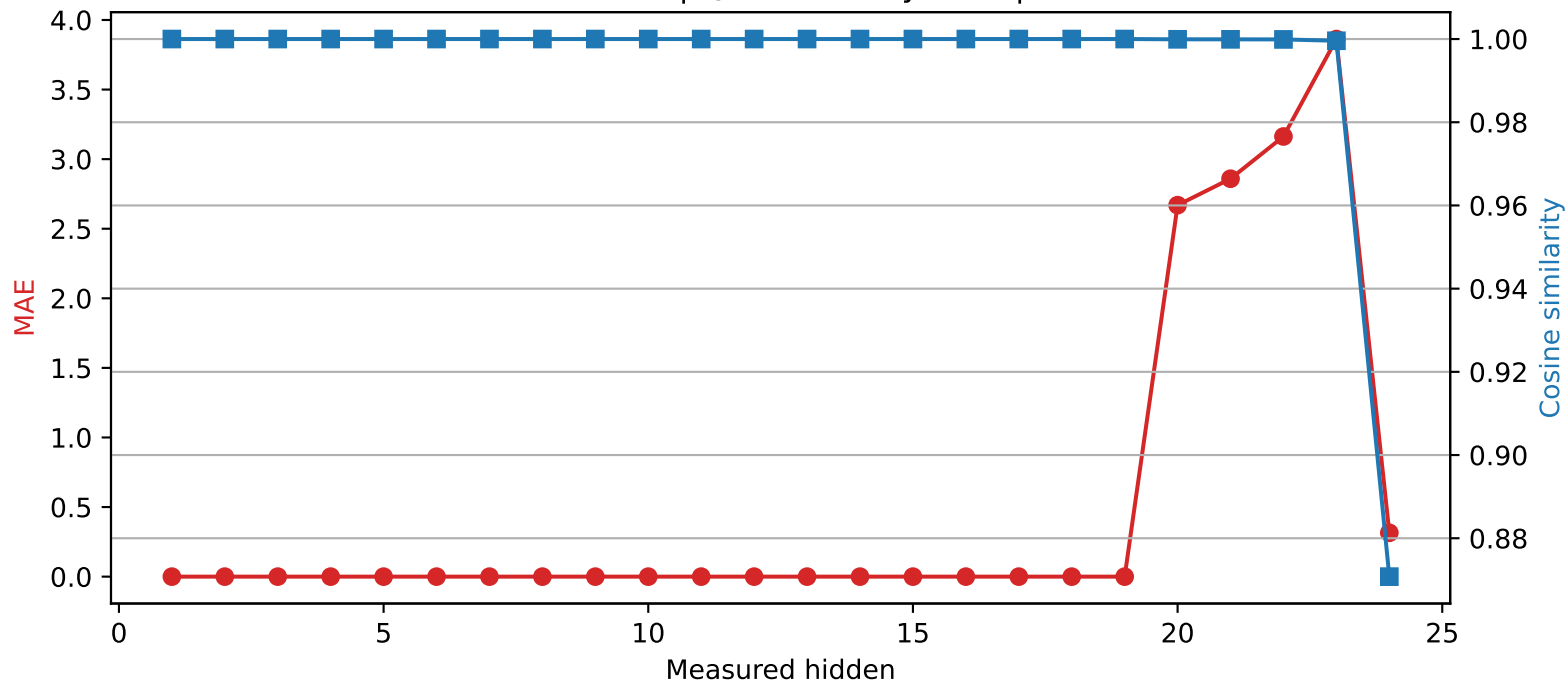
SmolLM2-1.7B-Instruct | Quantized layer 19 | float16 \rightarrow int4
