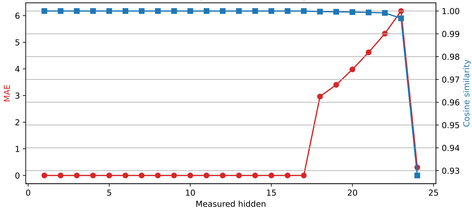
SmolLM2-1.7B-Instruct | Quantized layer 17 | float16 \rightarrow int4
