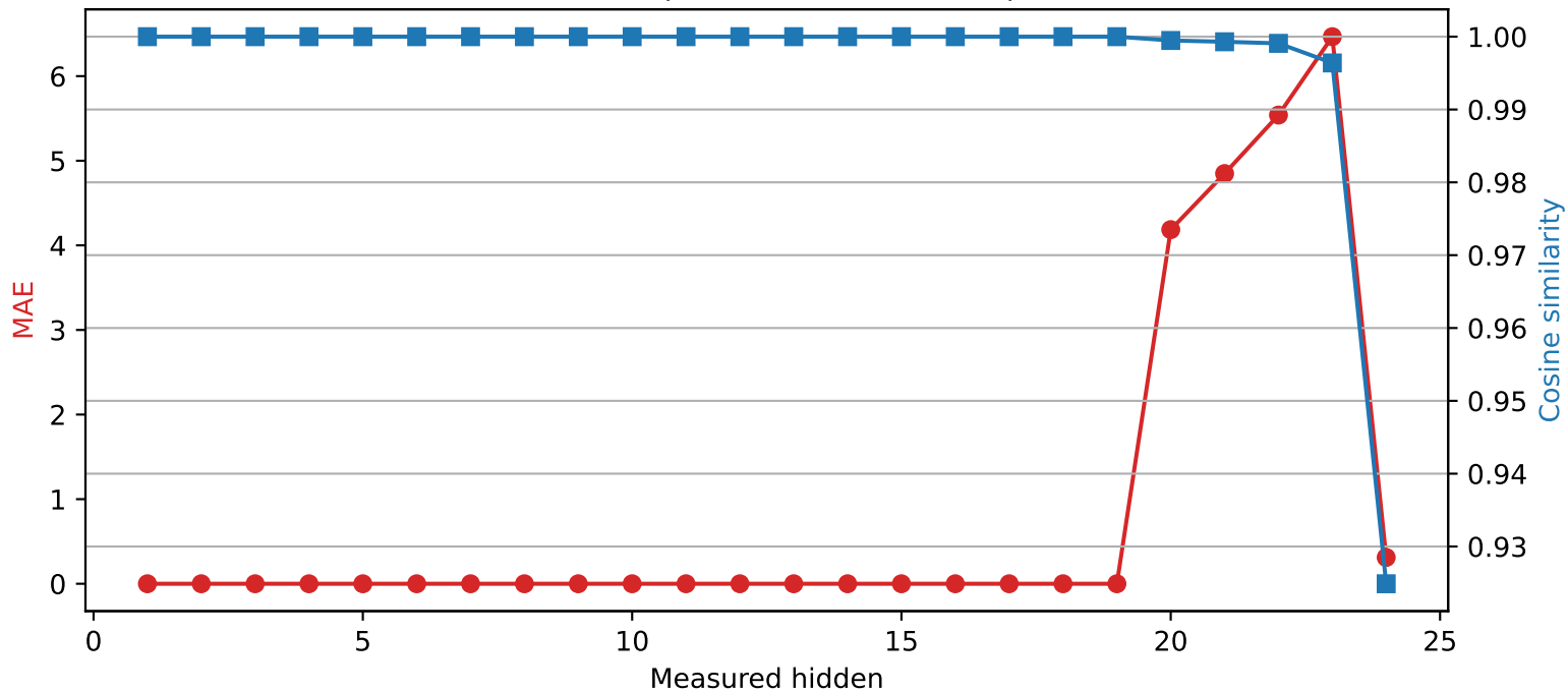
SmolLM2-1.7B-Instruct | Quantized layer 19 | float16 → int4
