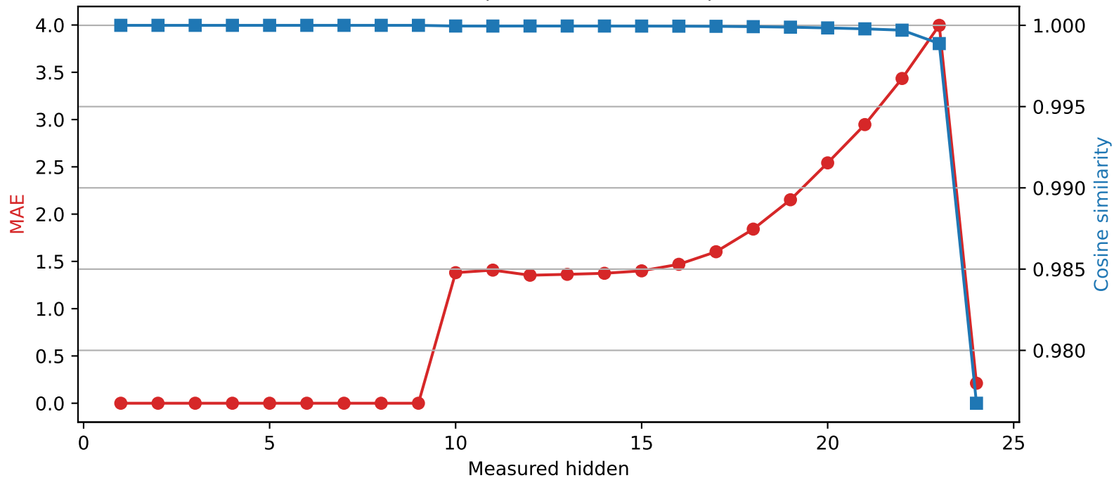
SmolLM2-1.7B-Instruct | Quantized layer 9 | float16 \rightarrow int4
