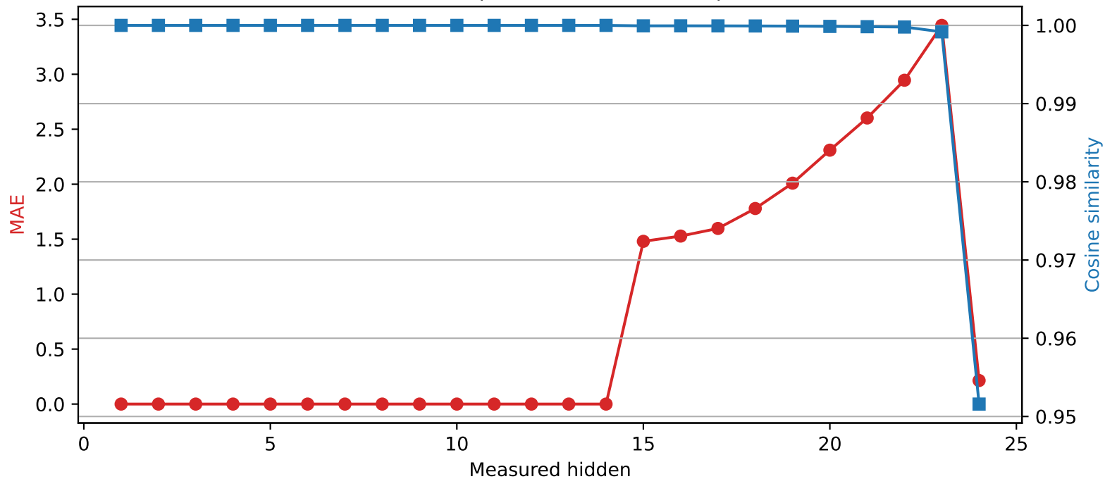
SmolLM2-1.7B-Instruct | Quantized layer 14 | float16 \rightarrow int4
