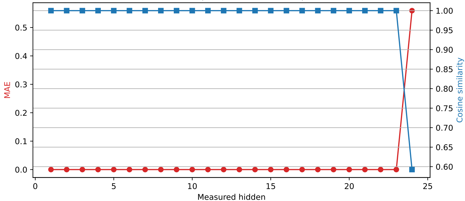
SmolLM2-1.7B-Instruct | Quantized layer 23 | float16 → int4
