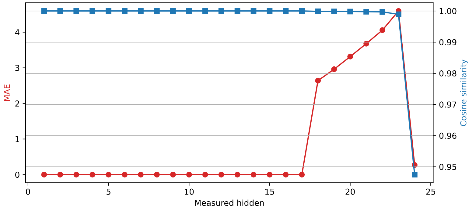
SmolLM2-1.7B-Instruct | Quantized layer 17 | float16 → int4
