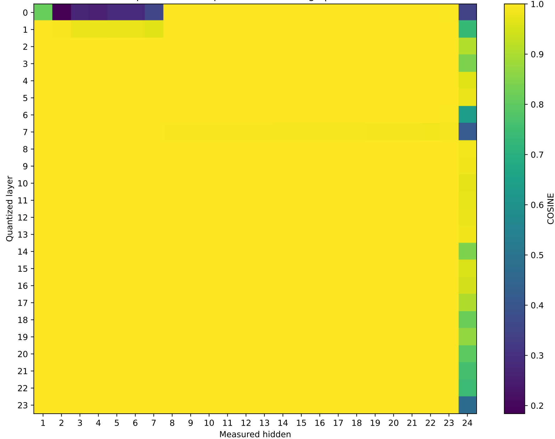
SmolLM2-1.7B-Instruct Prompt 0: cos sim representation damage | float32 → int4
