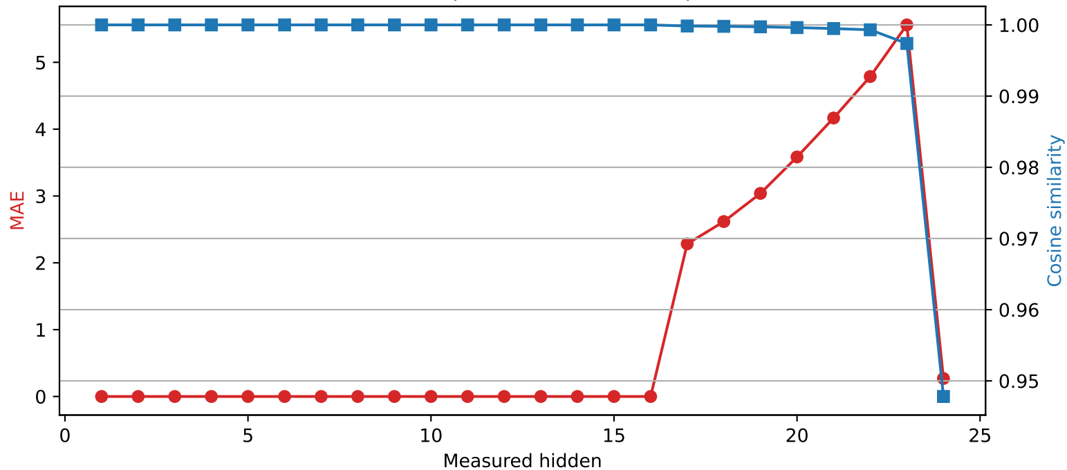
SmolLM2-1.7B-Instruct | Quantized layer 16 | float32 → int4
