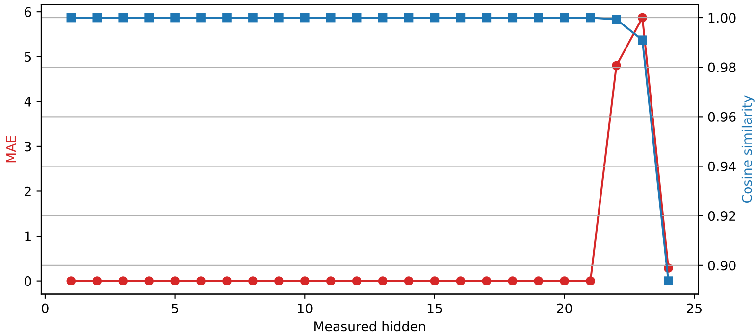
SmolLM2-1.7B-Instruct | Quantized layer 21 | float32 → int4
