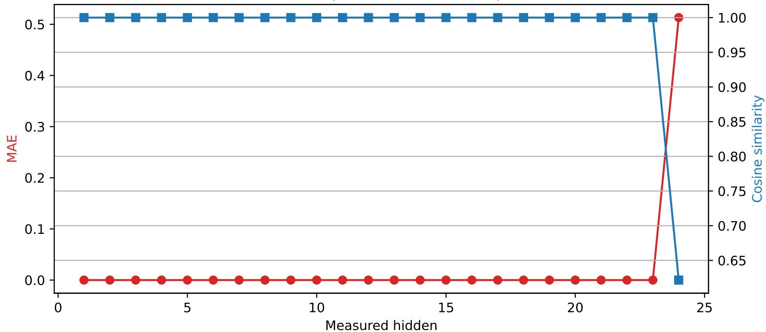
SmolLM2-1.7B-Instruct | Quantized layer 23 | float32 → int4
