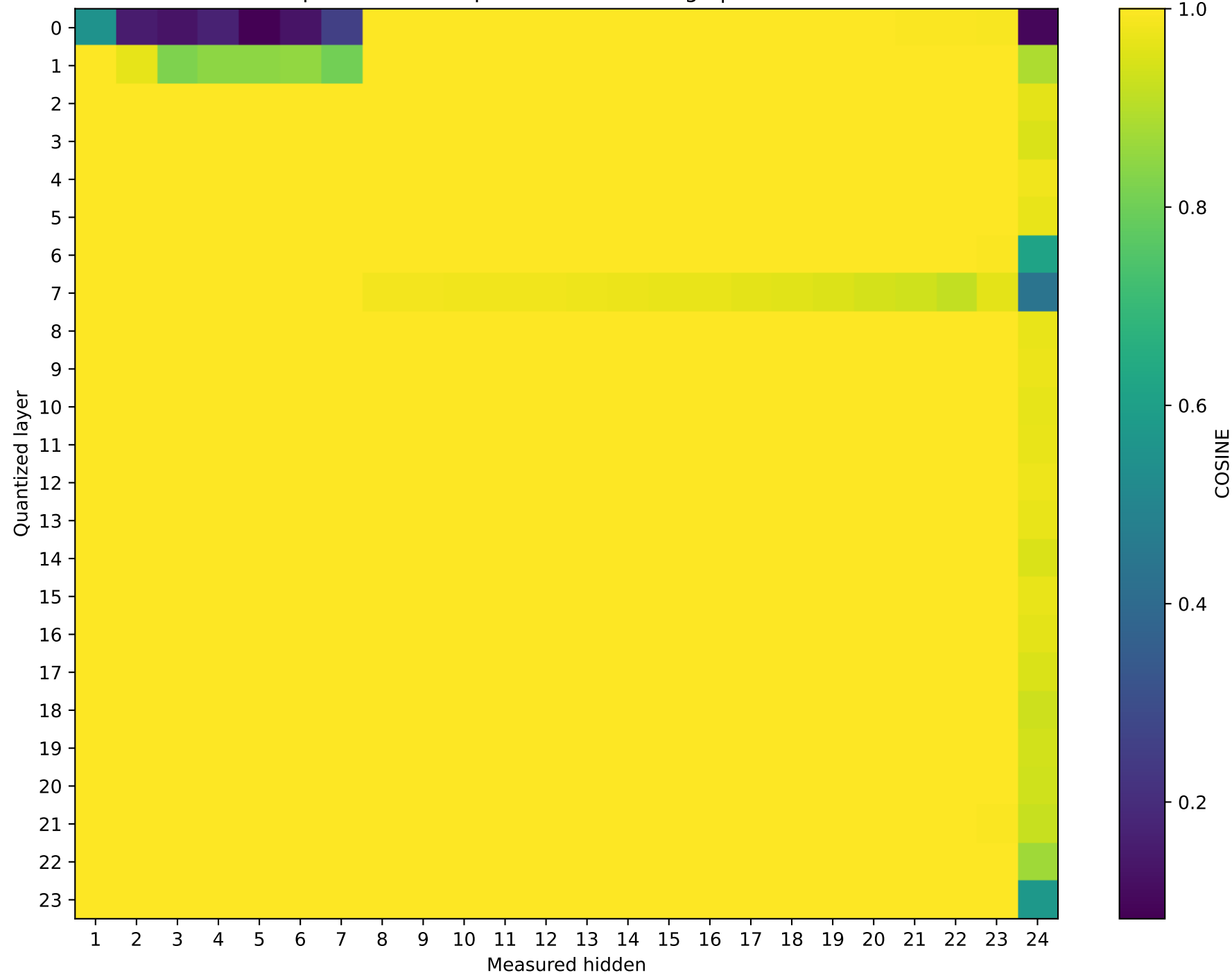
SmolLM2-1.7B-Instruct Prompt 4: cos sim representation damage | float32 → int4
