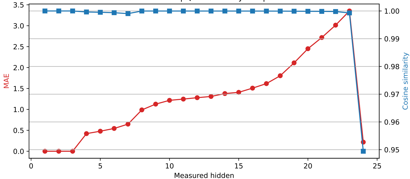
SmolLM2-1.7B-Instruct | Quantized layer 3 | float32 \rightarrow int4
