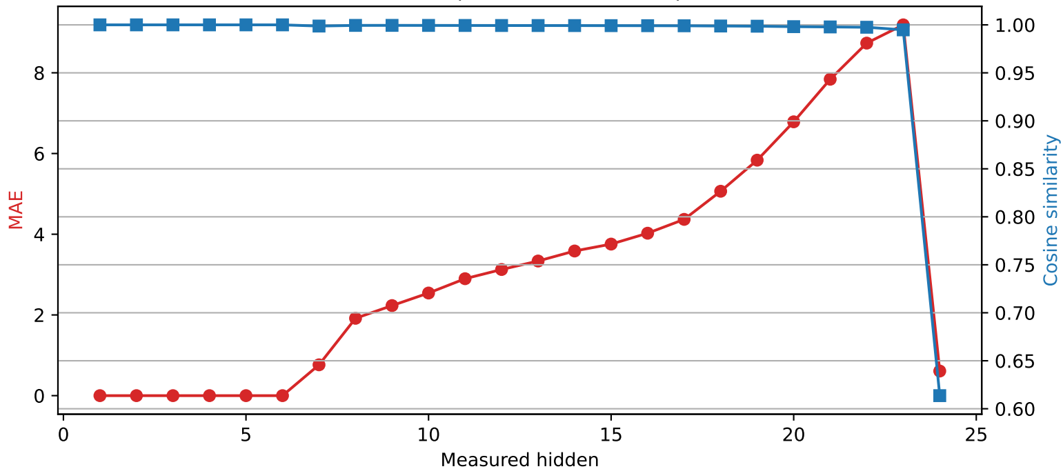
SmolLM2-1.7B-Instruct | Quantized layer 6 | float32 → int4
