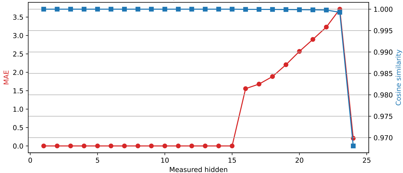
SmolLM2-1.7B-Instruct | Quantized layer 15 | float32 → int4
