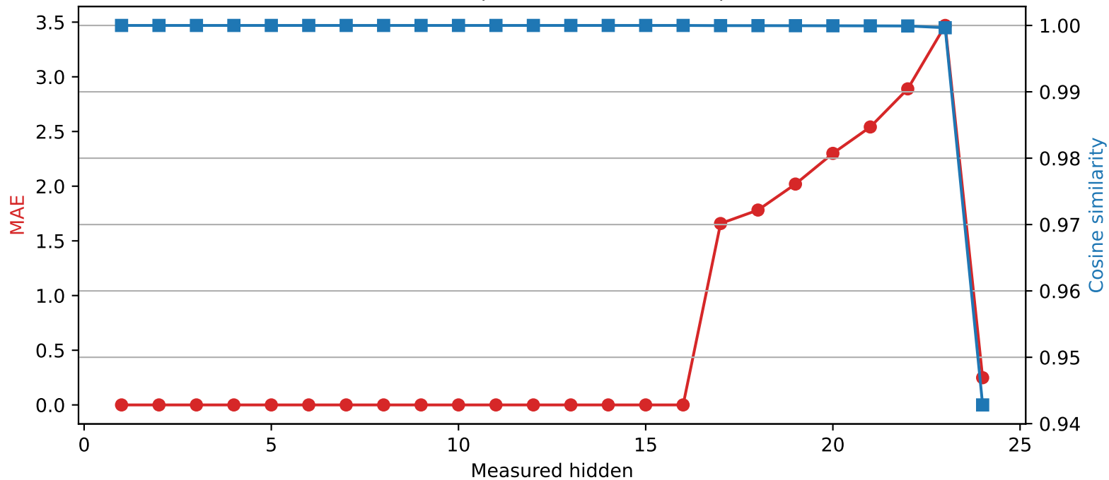
SmolLM2-1.7B-Instruct | Quantized layer 16 | float64 \rightarrow int4
