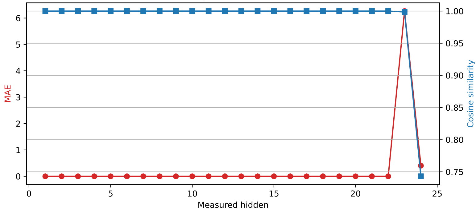
SmolLM2-1.7B-Instruct | Quantized layer 22 | float64 → int4
