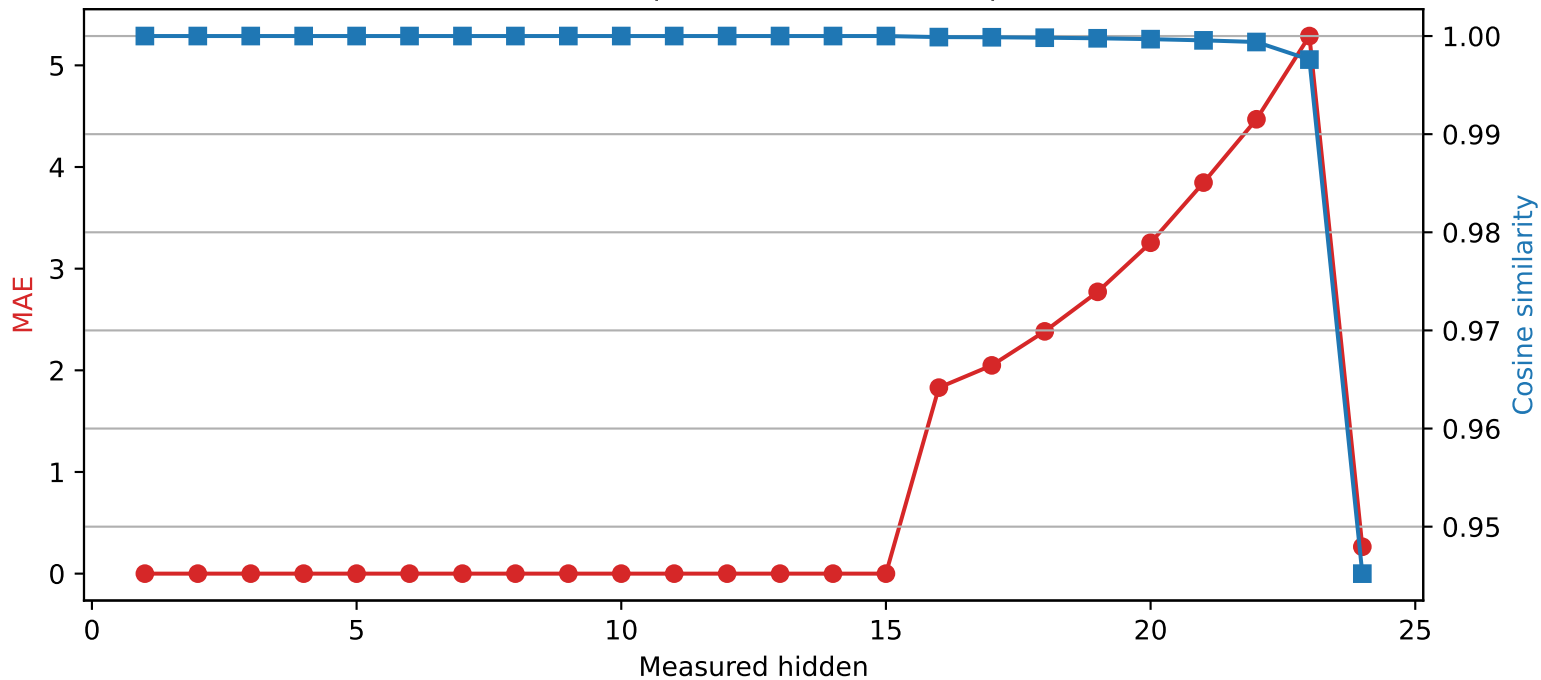
SmolLM2-1.7B-Instruct | Quantized layer 15 | float64 → int4
