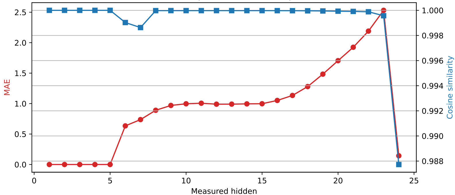
SmolLM2-1.7B-Instruct | Quantized layer 5 | float64 → int4
