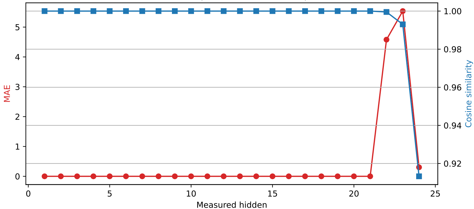
SmolLM2-1.7B-Instruct | Quantized layer 21 | float64 → int4
