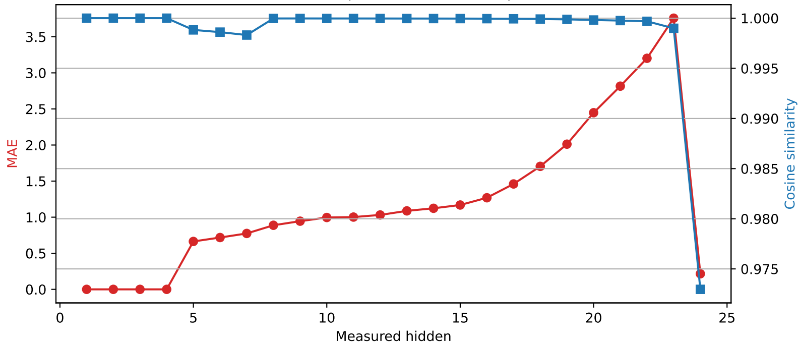
SmolLM2-1.7B-Instruct | Quantized layer 4 | float64 → int4
