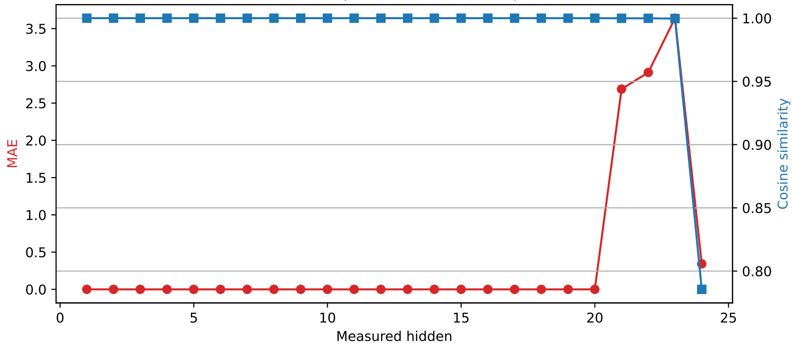
SmolLM2-1.7B-Instruct | Quantized layer 20 | float16 \rightarrow int2
