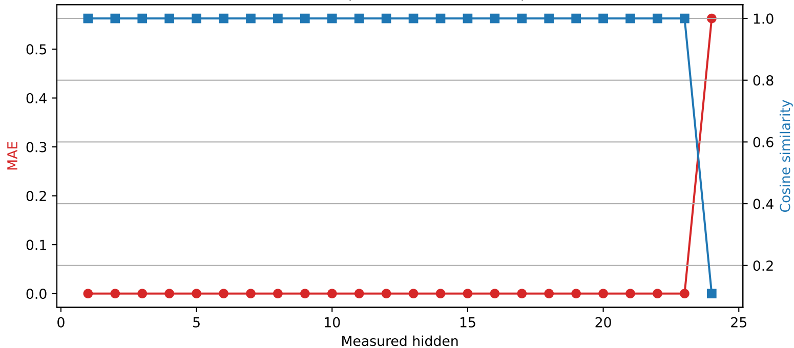
SmolLM2-1.7B-Instruct | Quantized layer 23 | float16 → int2
