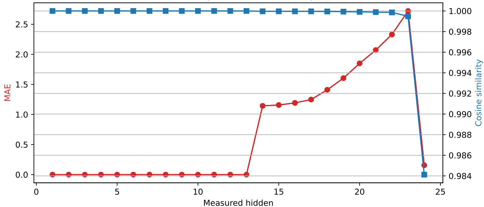
SmolLM2-1.7B-Instruct | Quantized layer 13 | float16 → int2
