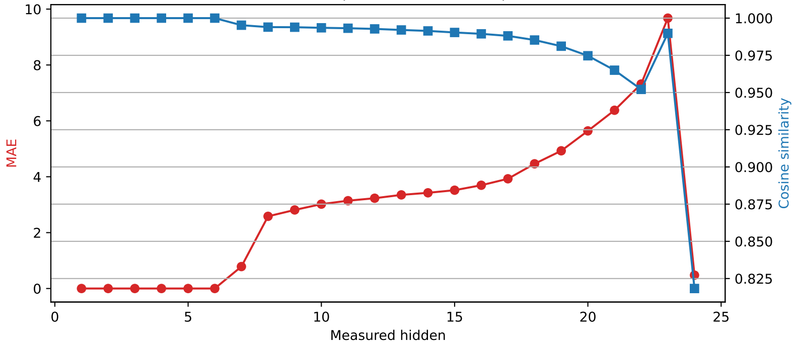
SmolLM2-1.7B-Instruct | Quantized layer 6 | float16 → int2
