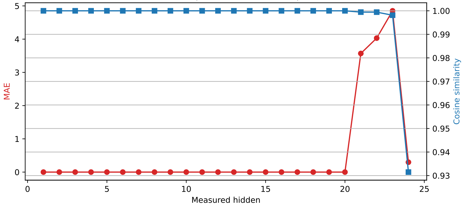
SmolLM2-1.7B-Instruct | Quantized layer 20 | float16 \rightarrow int2
