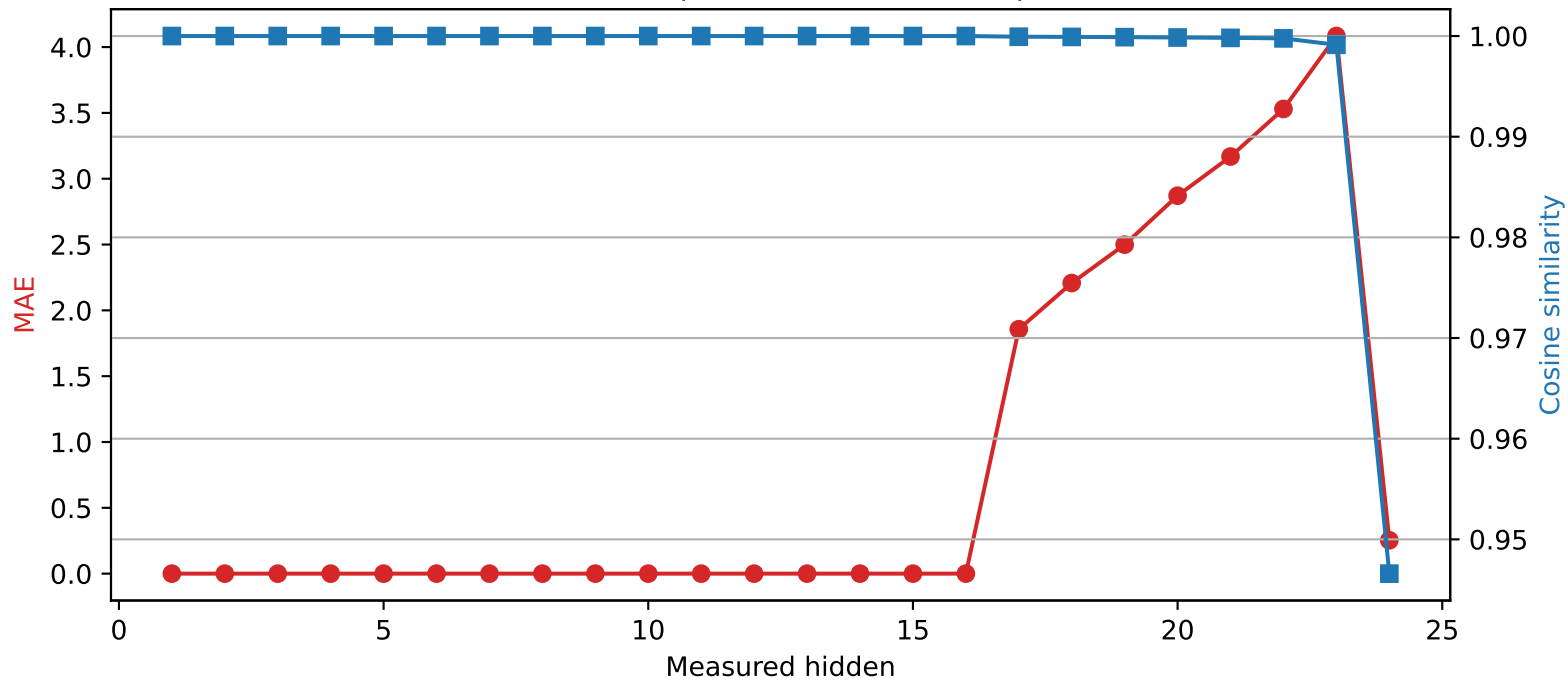
SmolLM2-1.7B-Instruct | Quantized layer 16 | float16 → int2
