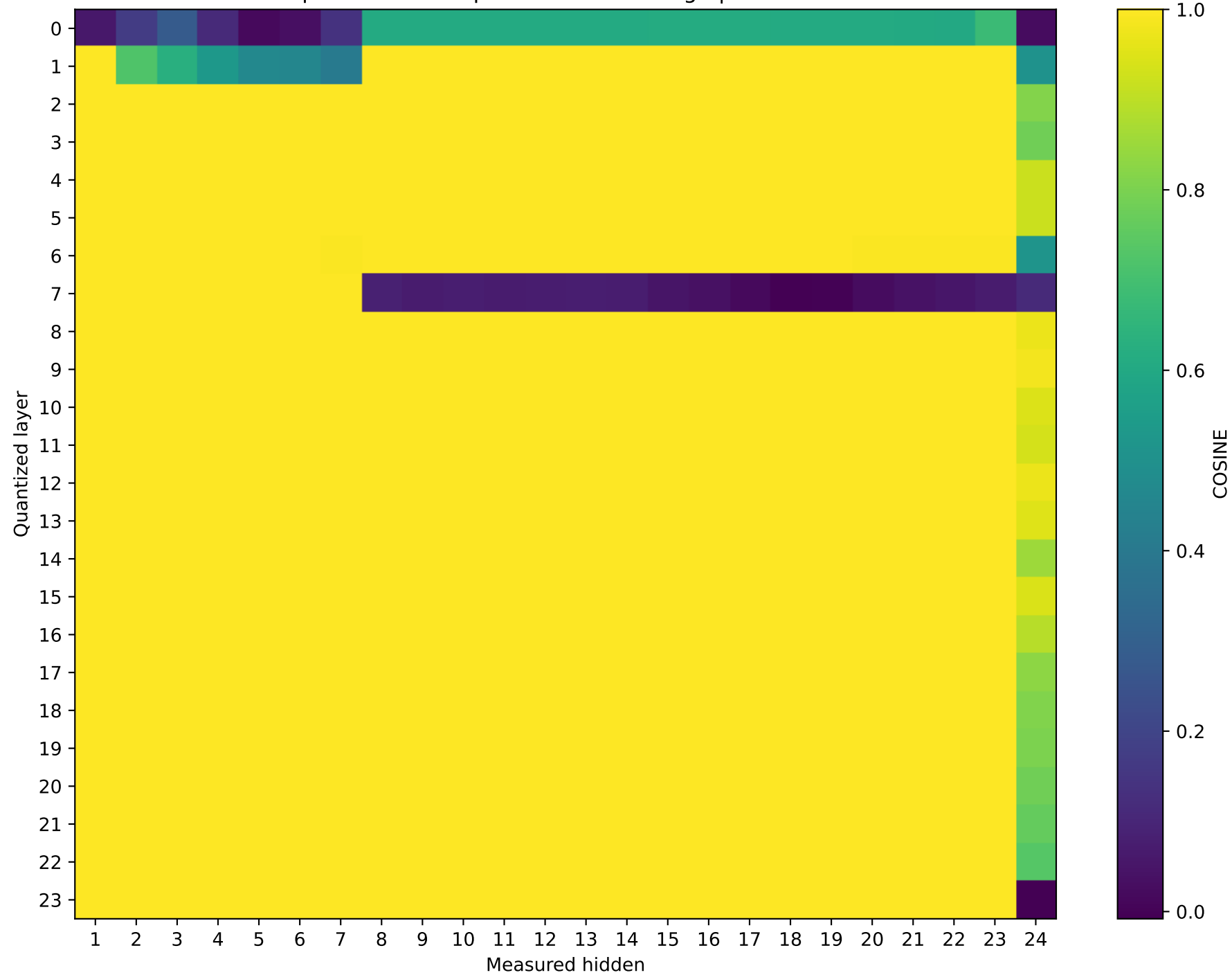
SmolLM2-1.7B-Instruct Prompt 0: cos sim representation damage | float32 → int2
