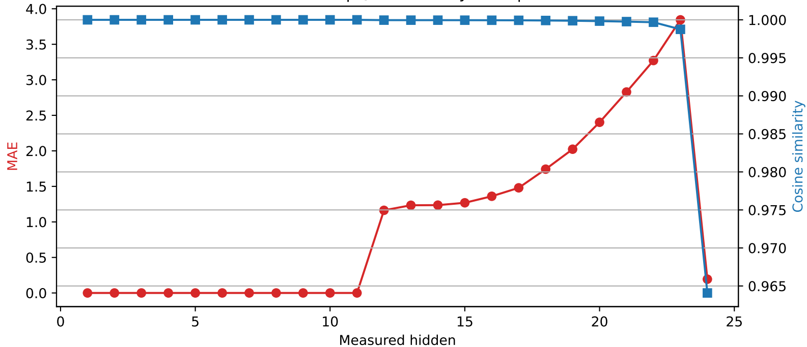
SmolLM2-1.7B-Instruct | Quantized layer 11 | float32 → int2
