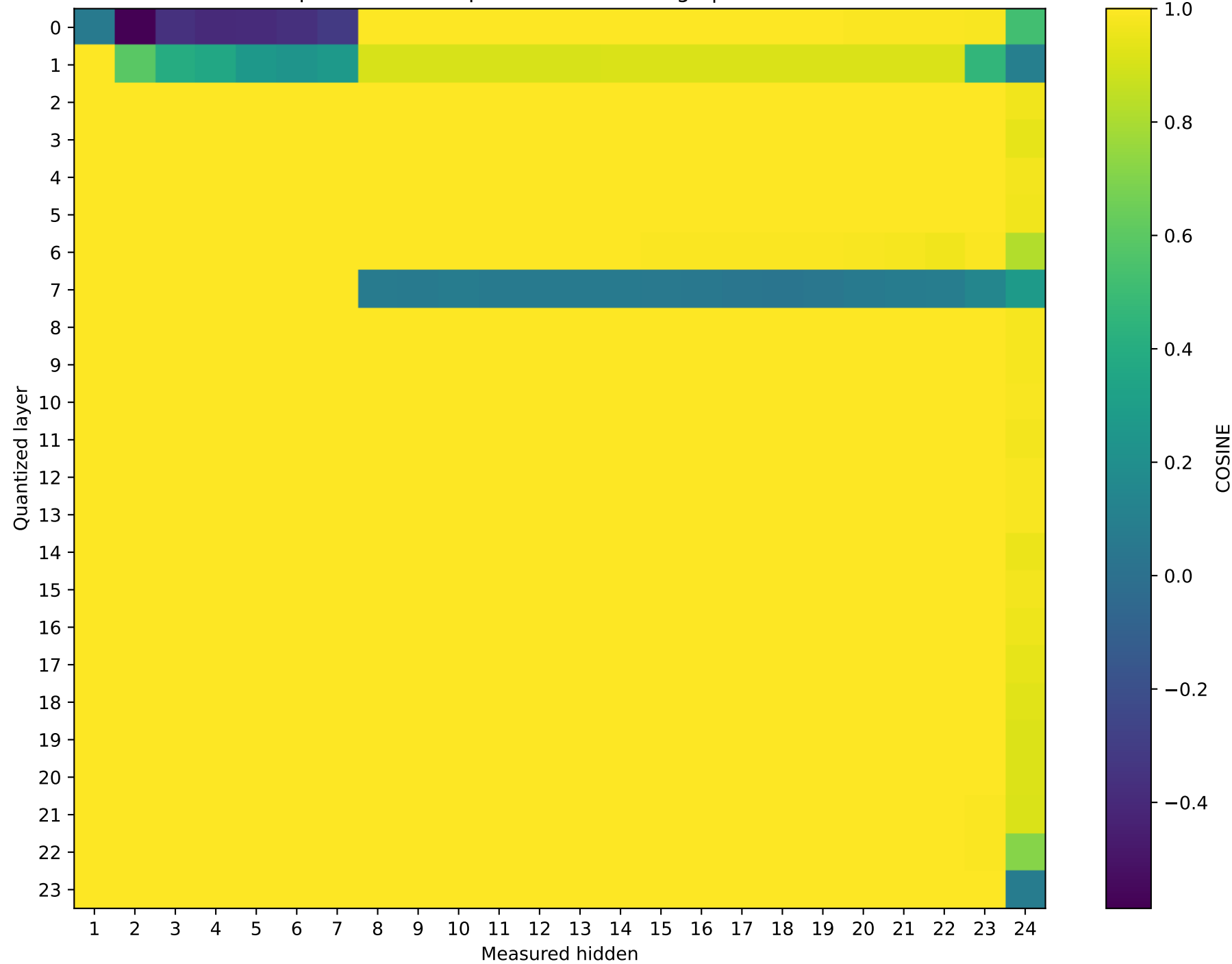
SmolLM2-1.7B-Instruct Prompt 2: cos sim representation damage | float32 → int2
