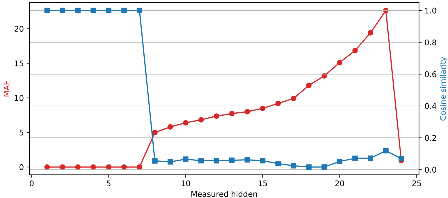
SmolLM2-1.7B-Instruct | Quantized layer 7 | float32 \rightarrow int2
