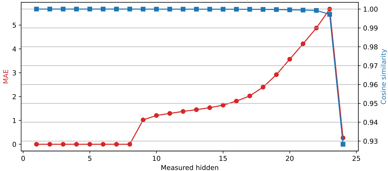
SmolLM2-1.7B-Instruct | Quantized layer 8 | float64 → int2
