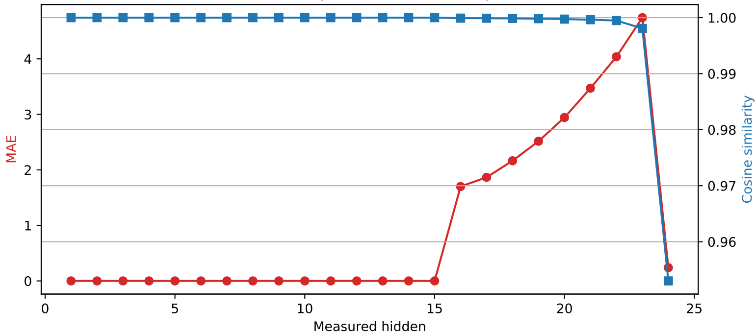
SmolLM2-1.7B-Instruct | Quantized layer 15 | float64 → int2
