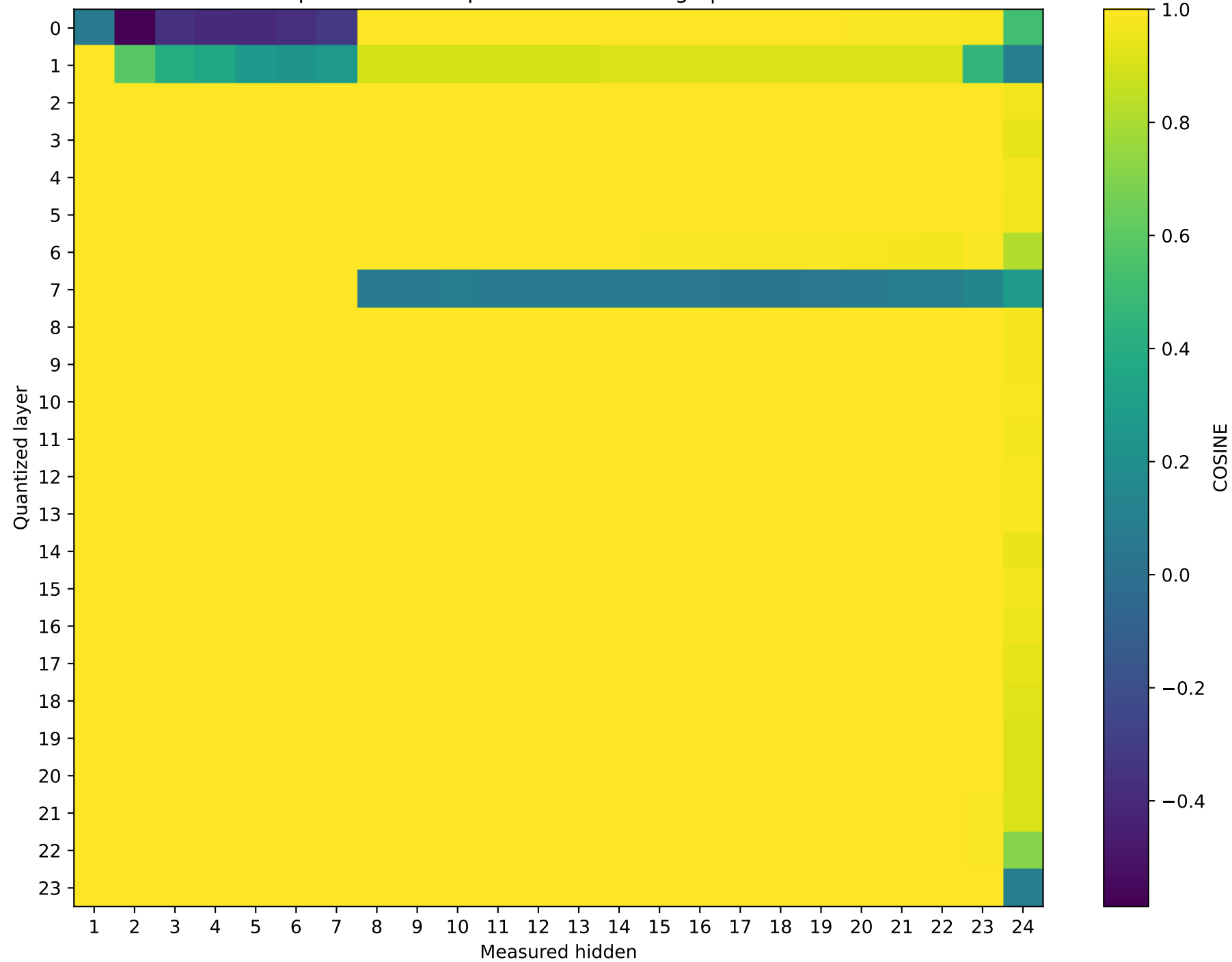
SmolLM2-1.7B-Instruct Prompt 2: cos sim representation damage | float64 → int2
