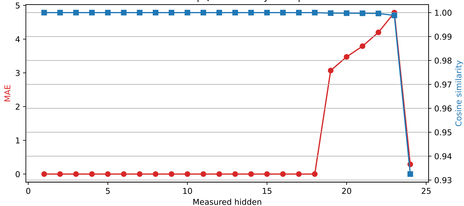
SmolLM2-1.7B-Instruct | Quantized layer 18 | float64 → int2
