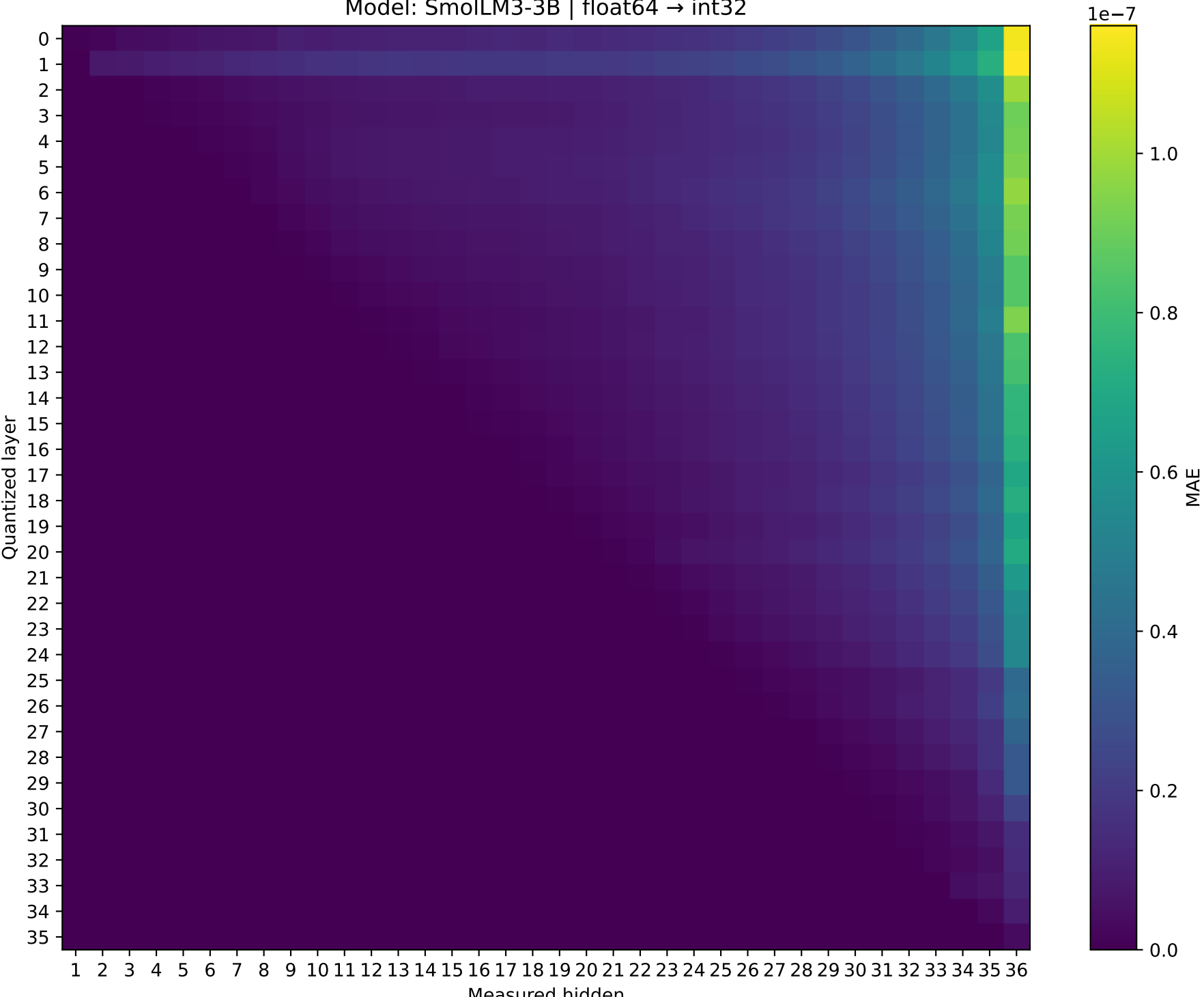
Model: SmolLM3-3B | float64 → int32
