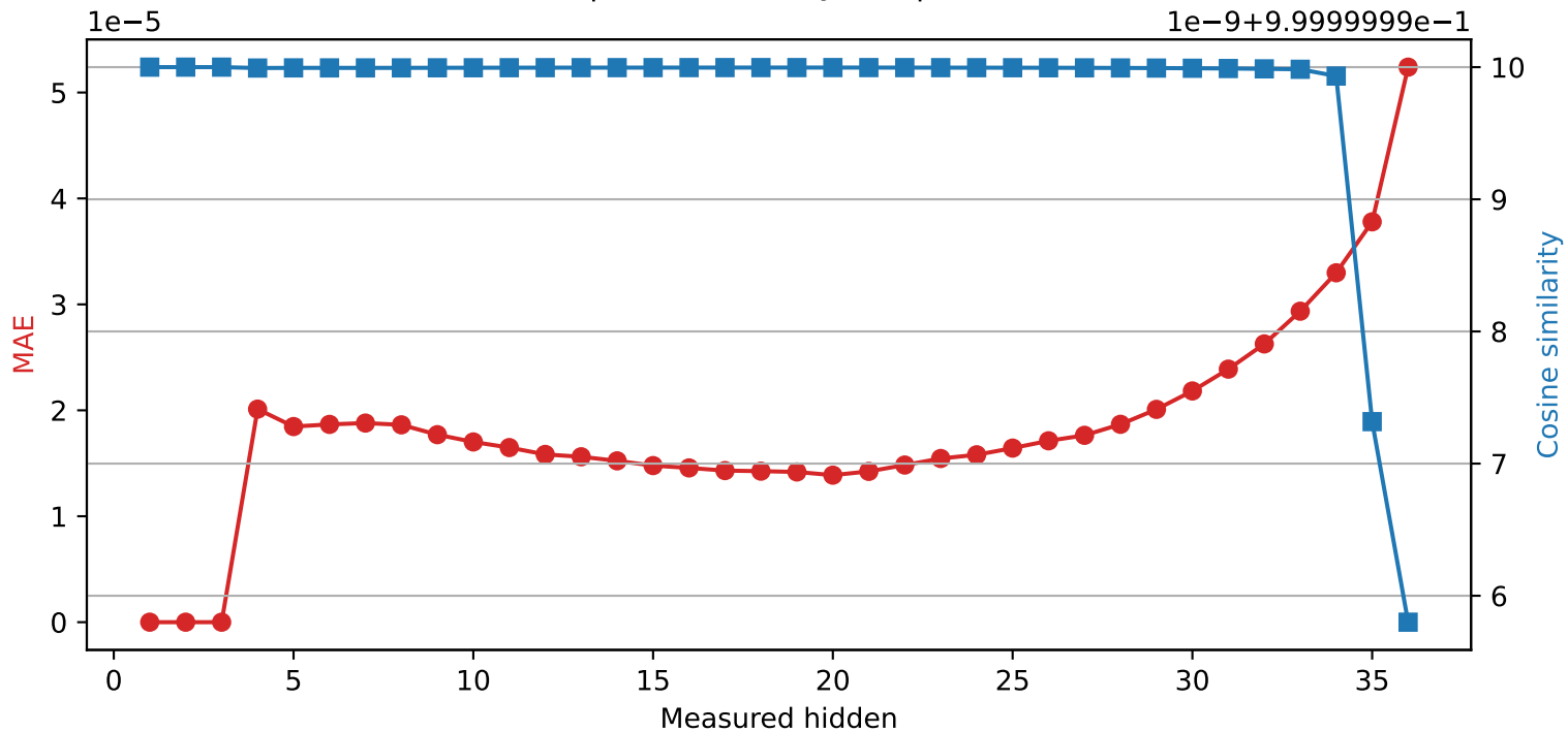
SmolLM3-3B | Quantized layer 3 | float32 → int16
